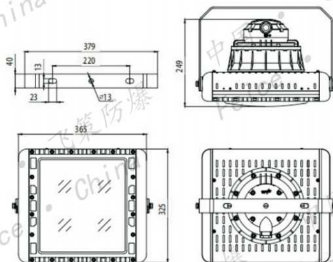
FCF(T)98-(200W-240W)
