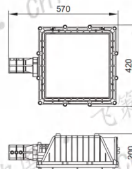
II 型/路灯/分体式 II Type/Street lamp type/red-tipped
