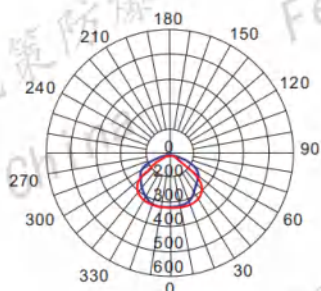
I 型: 金卤灯 175W Source: 175W Metal halide lamp — c0/180 — c90/270 cd/1000lm
