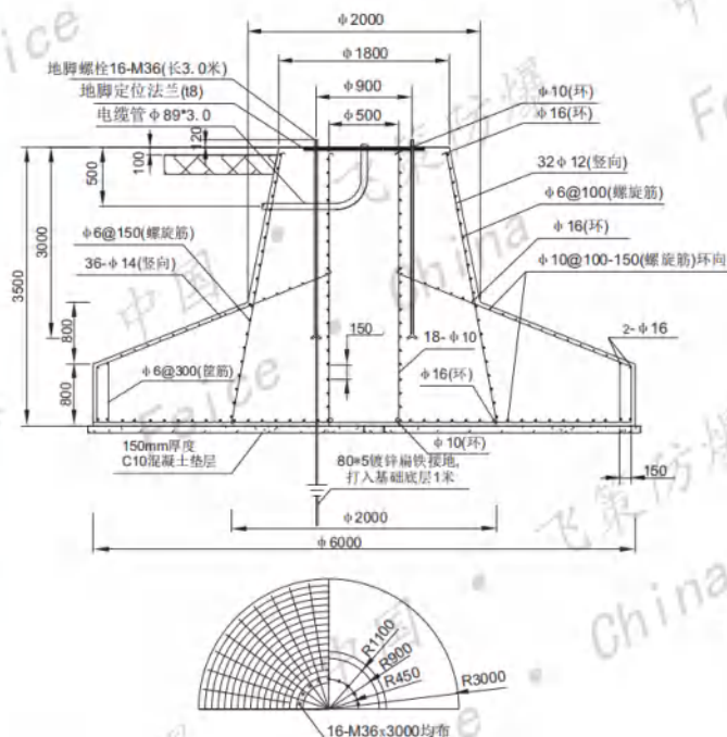
35m高杆灯 High-pole lamp 基础平面图 Foundation plan
