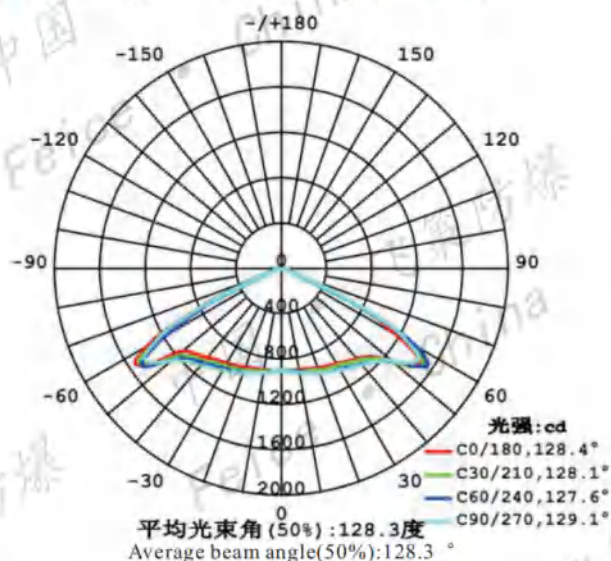
■ 配光曲线 Luminous distribution curve
