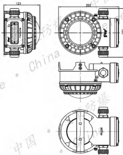
FC-ZFJC-E9W 壁式、吸顶式 FC-ZFJC-E9W wall type, ceiling type
