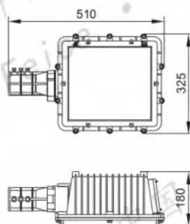
I 型/路灯分体式 I Type/Street lamp type/red-tipped
