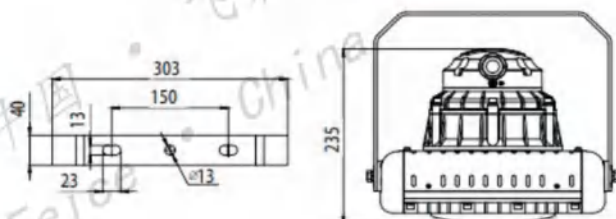
FCF98-(80W-100W)
