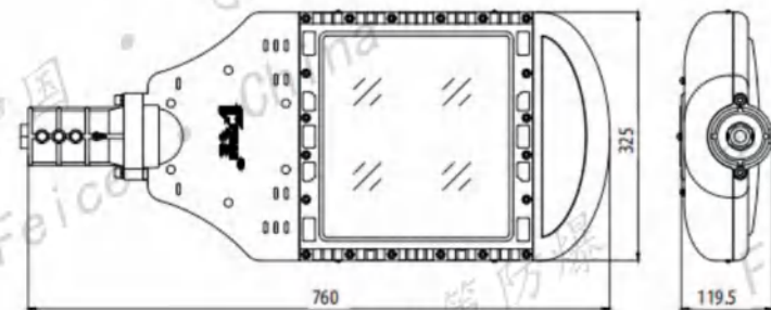
FCL98-(200W-240W)
