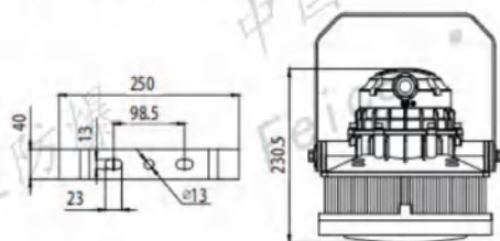
FCL98-(200W-240W)
