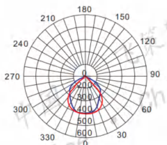
II 型: 金卤灯 400W Source: 400W Metal halide lamp — c0/180 — c90/270 cd/1000lm
