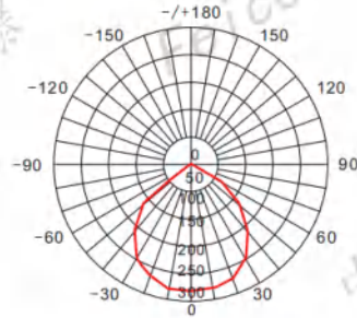
IV 型: 金卤灯 400W Source: 400W Metal halide lamp cd/3000lm
