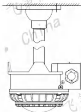
FC-ZFJC-E9W 吊杆式 FC-ZFJC-E9W boom type
